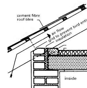
⑨ Pitched roof with solid ceiling
